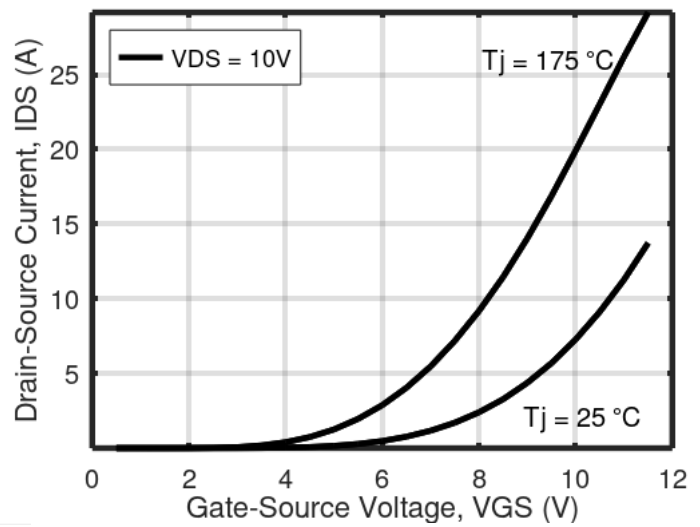
Figure 6: Transfer Characteristic For Two Temperatures
