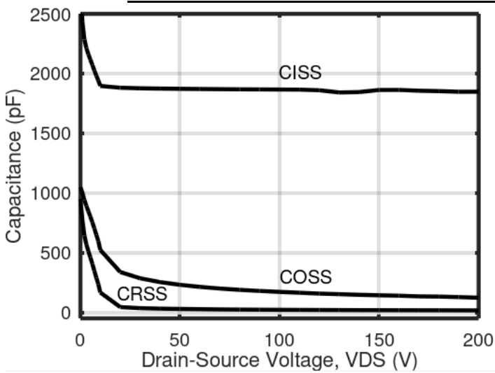
Figure 5: Capacitances vs. Drain-Source Voltage (0 - 200V), VGS = 0 V
