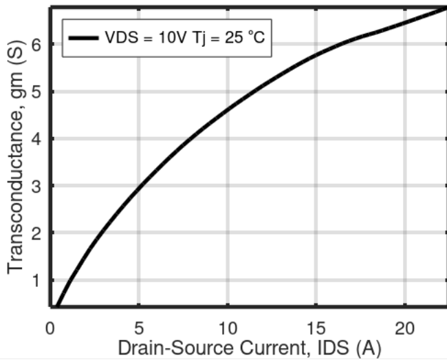
Figure 7: Transconductance vs. Drain Current
