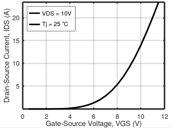
Figure 6: Transfer Characteristic
