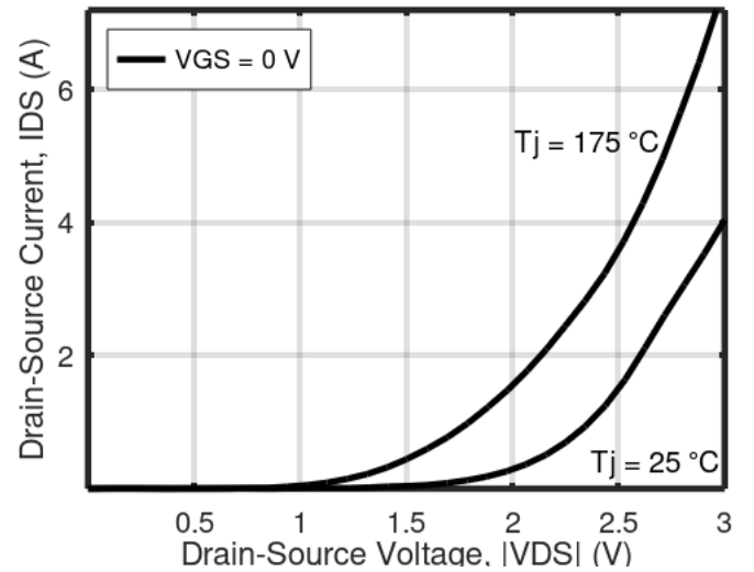
Figure 8: Body Diode Characteristic For Various Temperatures
