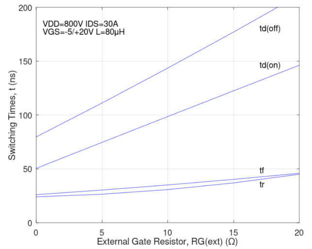
Figure 23: Clamped inductive switching energy vs. temperature. Figure 24: Switching times vs. external gate resistance.
