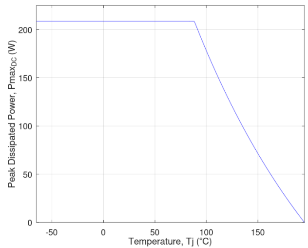
Figure 20: Power dissipation derating vs. temperature.
