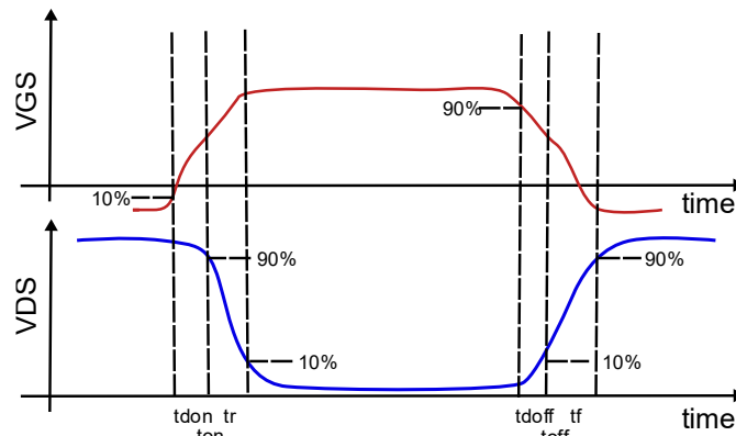
Figure 25: Timing references.
