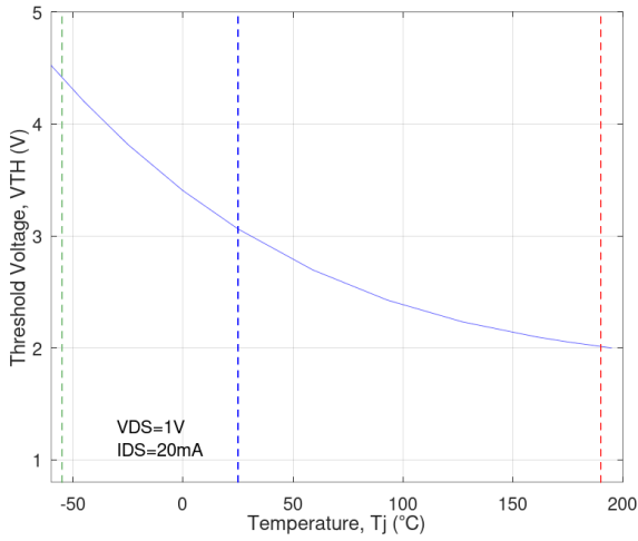
Figure 11: Threshold vs. temperature.
