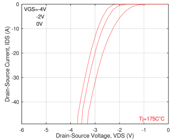
Figure 10: High temperature body diode characteristics†.
