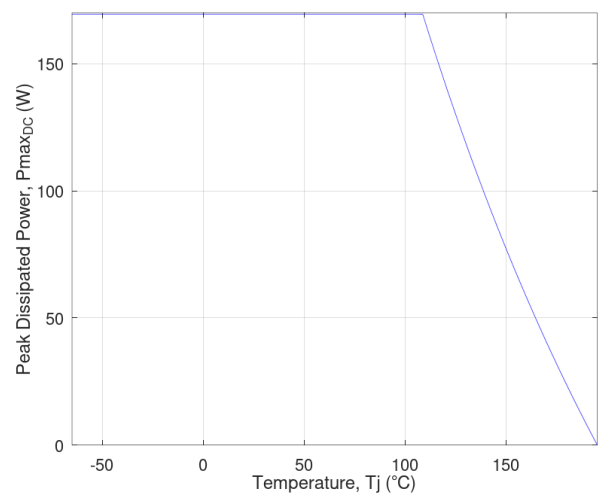
Figure 20: Power dissipation derating vs. temperature. (IDS=80A)
