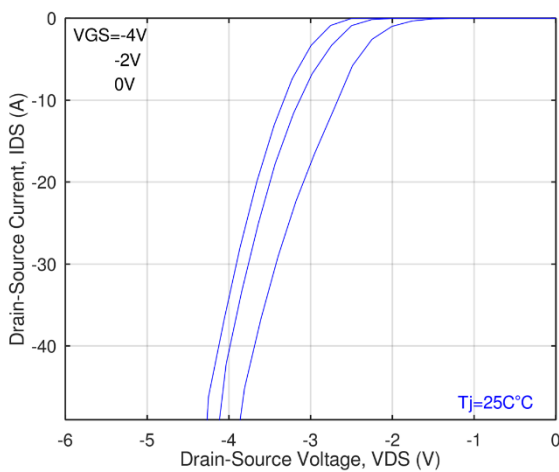
Figure 9: Room temperature body diode characteristics†.
