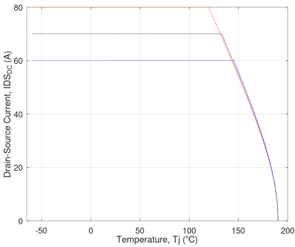
Figure 19: Continuous drain current vs. temperature.
