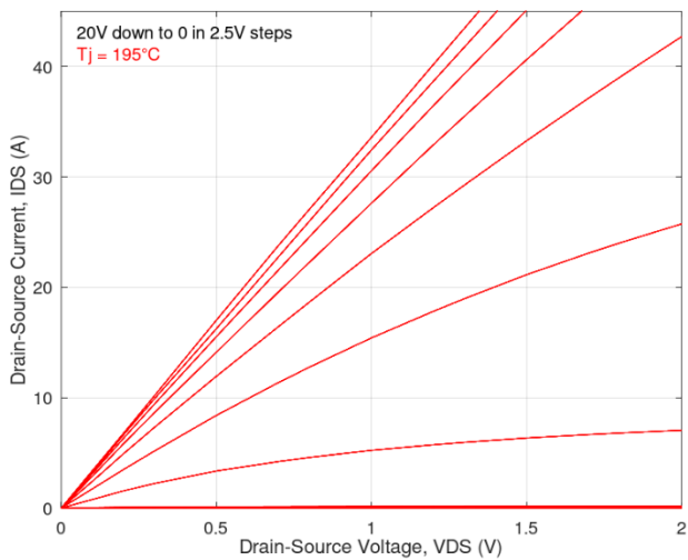
Figure 3: High temperature output characteristics†.
